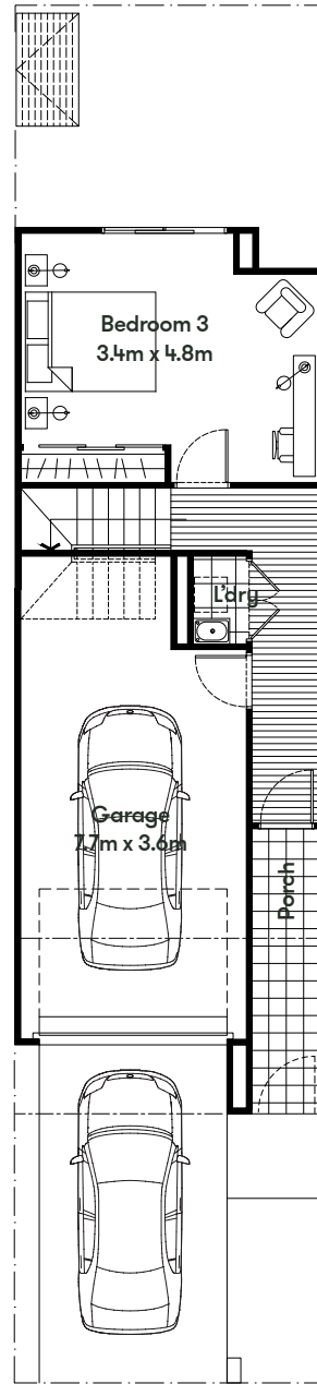
GROUND FLOOR
